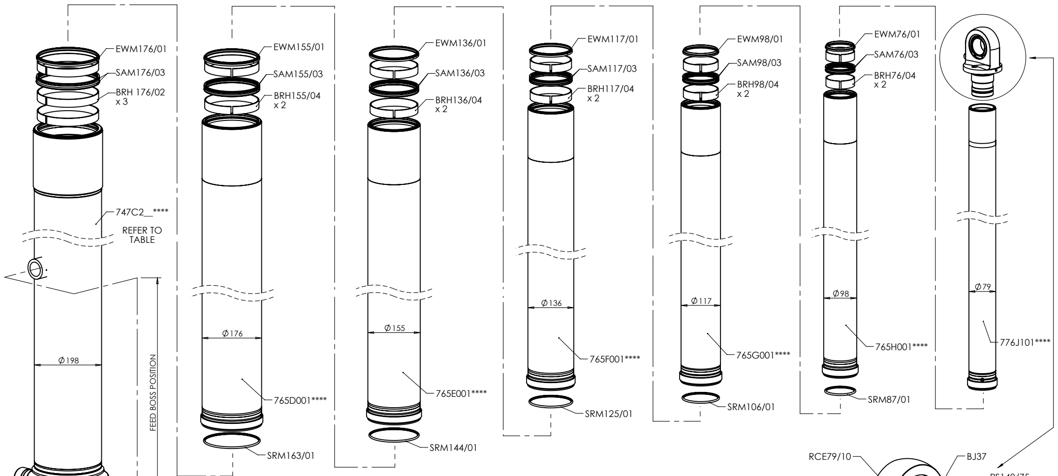
Base Tube Selection Table
