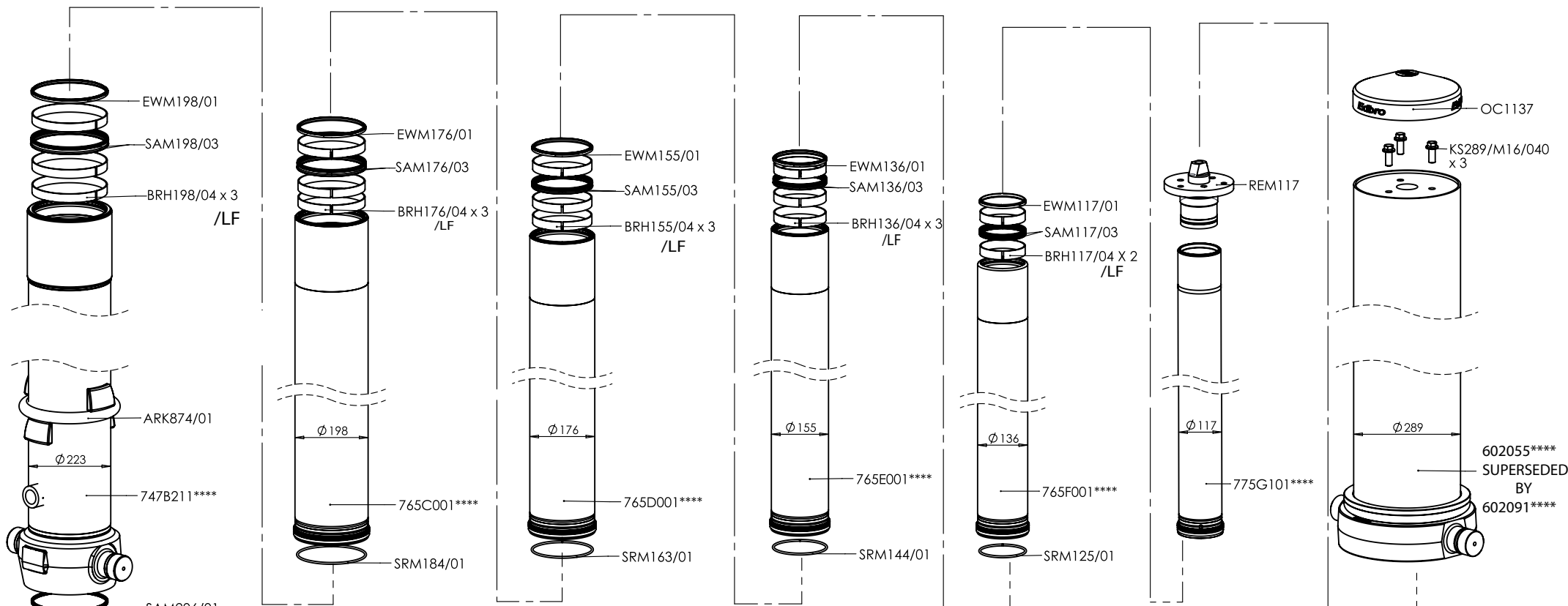
Base Tube Selection Table
